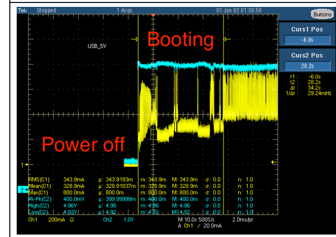
Fig 9: USB_5V Booting
